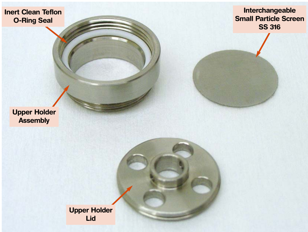
Upper Holder Assembly Overview
