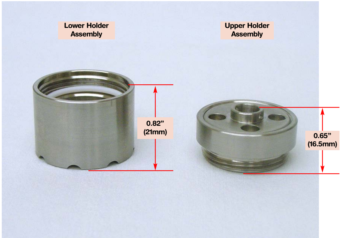
Small Particle Holder Overview
